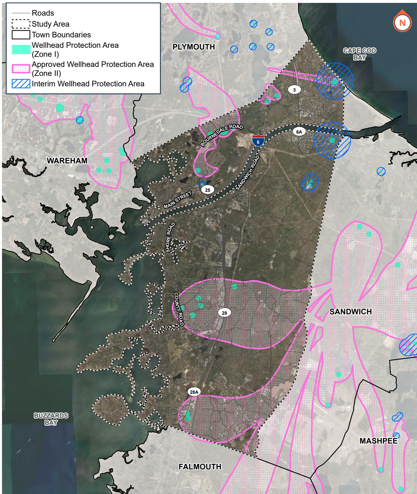
Figure 6 CWMP - Groundwater Constraints Bourne, Massachusetts
